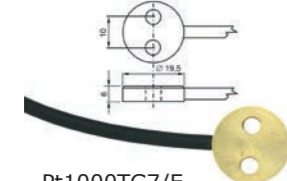
Pt1000TG7/E (-30°C to +200°C)
